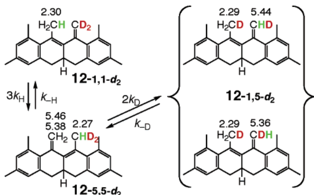
Figure 2. Kinetic scheme for the interconversions starting from 12-1,1- d 2 are shown along with the 1 H NMR signals employed in the analyses of concentrations versus time.
