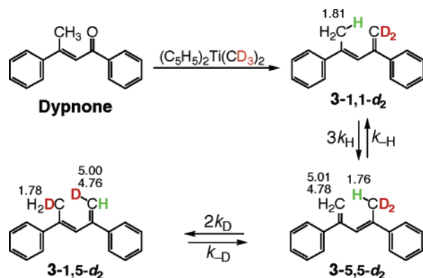
Figure 1. Preparation from dyppone of 3-1,1- d 2 and its thermal rearrangement to 3-5,5- d 2 and 3-1,5- d 2 are shown. The shifts in the 1 H NMR spectrum of the hydrogen atoms used in the analysis of the kinetics are shown in ppm ( \delta ).
