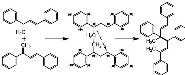
Figure 1. Preparation from dyppone of 3-1,1- d 2 and its thermal rearrangement to 3-5,5- d 2 and 3-1,5- d 2 are shown. The shifts in the 1 H NMR spectrum of the hydrogen atoms used in the analysis of the kinetics are shown in ppm ( \delta ).
