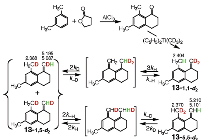
Figure 3. Preparation and kinetic profile of 6,8-dimethyl-1-dideuteriomethylene-1,2,3,4-tetrahydronaphthalene are depicted. The 1 H NMR used in quantitative analysis are given in ppm ( \delta ) above the relevant groups.
